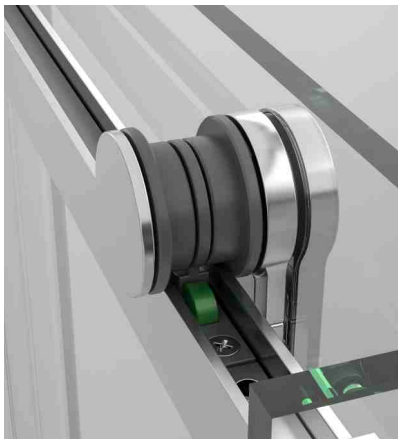
Buffer and roller contact detail image
