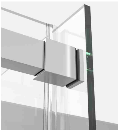
S131 corner connector detail image
