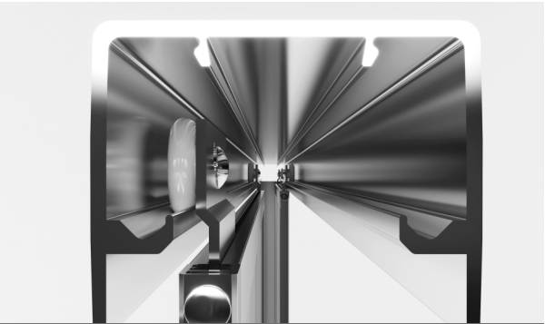
Upper rail cross-section detail image
