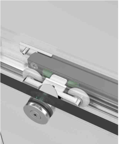
Buffer and roller contact detail image
