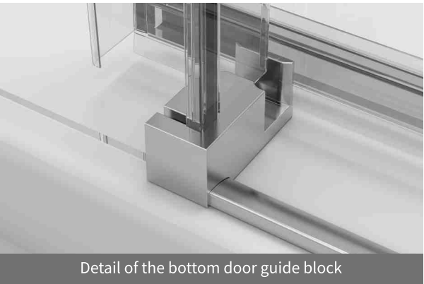
Detail of the bottom door guide block
