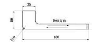
ZFG5 厕纸架 Roll Paper Holder 180*50*50mm
