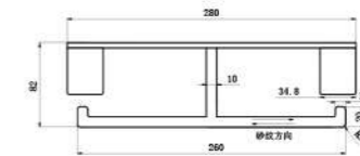
ZFG8S 带置物双纸巾架 Double Paper Holder with cover 280*100*80mm
