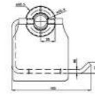
JT06 Paper holder 纸巾架 (带盖)
