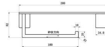
ZFG8 带置物纸巾架 Paper towel holder with slot 200*100*80mm
