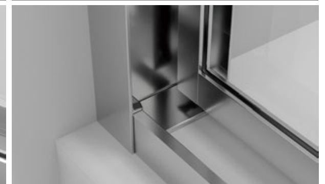
Plastic cover design detail at the bottom rail and vertical material connection
