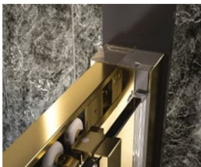
TOP RAIL DETAILS IN CLOSING POSITION
