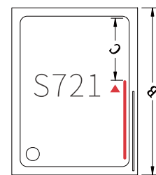
TOP RAIL DETAILS IN CLOSING POSITION
